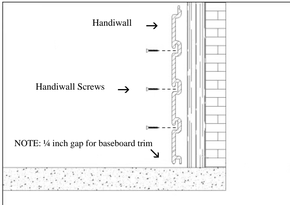
Figure 2. HANDIWALL installation.
